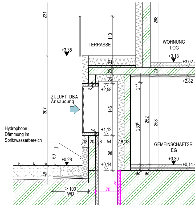
K6-K6
