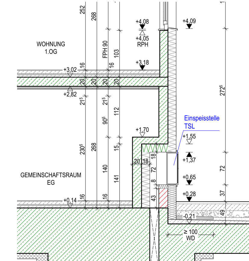
K5-K5
