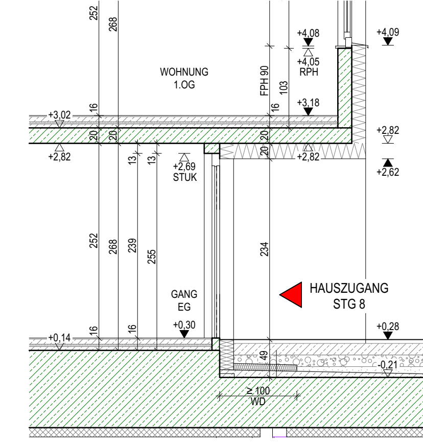
K4-K4
